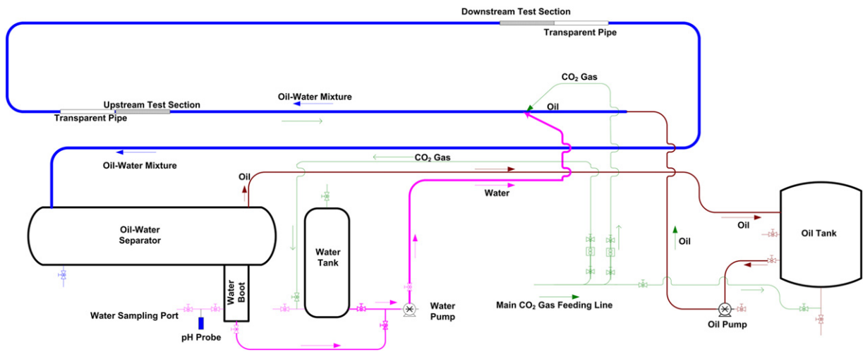
Fig. 3. Schematic of the inclinable flow loop used for the research. Oil and water are pumped separately and join in a 0.1 m pipe with a test section a and a transparent section located at the end of a 14 m straight pipe section.
