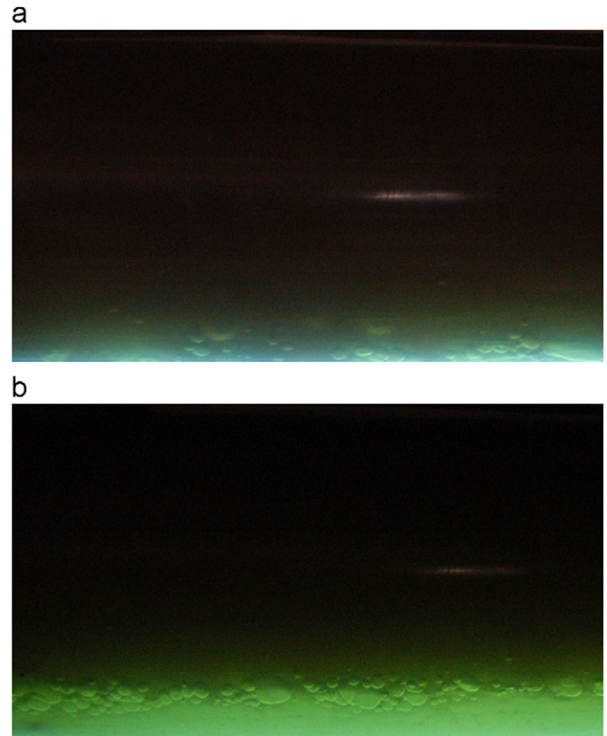
Fig. 9. Visualization of typical flow patterns at V_{st} = 0.5 m/s, taken under UV light with fluorescein salt added to the water. (a) At V_{sw} = 0.025 m/s (5% water cut) the water flows as globules at the bottom, (b) at V_{sw} = 0.1 m/s (20% water cut) the flow is stratified with a mixing layer on top of the water layer.
