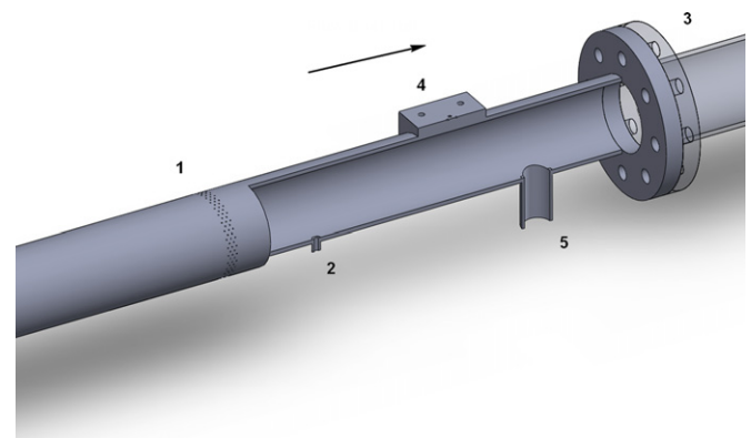
Fig. 5. Schematic of the test section showing the location of the different testing equipments with an arrow showing the direction of the flow. The equipment is located as follows: 1. Ports for conductivity pins, 2. Fluid sampling port, 3. Transparent pipe, 4. Saddle for High Frequency Impedance Probe and 5. Port for Electrical Resistance (ER) probe. The current study makes use of the conductivity pins, the wall sampling port and the transparent pipe.
