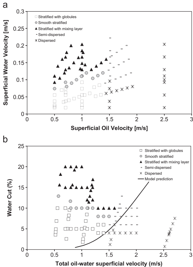
Fig. 8. Flow regime map of LVT200 oil–water flow in large diameter (0.1 m) horizontal pipe. The data is displayed in two ways (a) using superficial velocities and (b) using water cut and the total oil and water superficial velocity. The model prediction is included in the latter.
