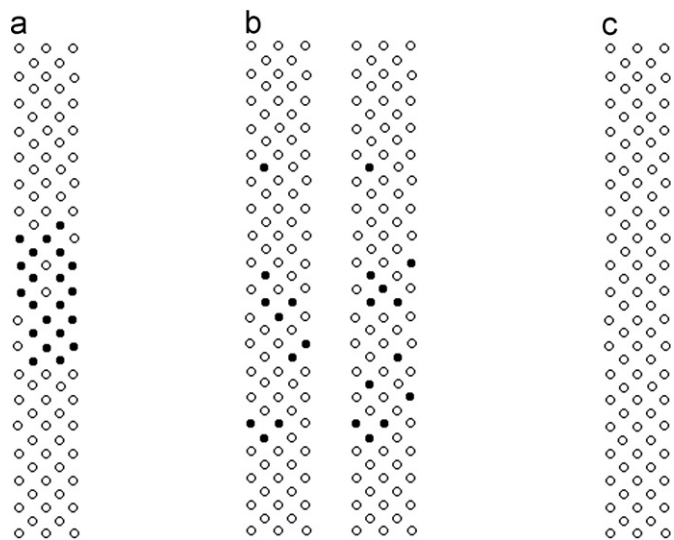
Fig. 7. Typical data for the conductivity pins distributed at the bottom half of the test section. It is displayed as a snapshot of simultaneous wetting of the pins, where an empty circle denotes oil wetting and a filled circle water wetting. The snapshots describe (a) stable water wetting, (b) intermittent wetting and (c) stable oil wetting. The bottom of the pipe corresponds to the vertical center of the pin snapshot.
