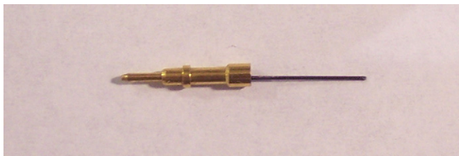
Fig. 6. One of the 160 conductivity pins, which are flush mounted on the internal wall of the mild steel test section.
