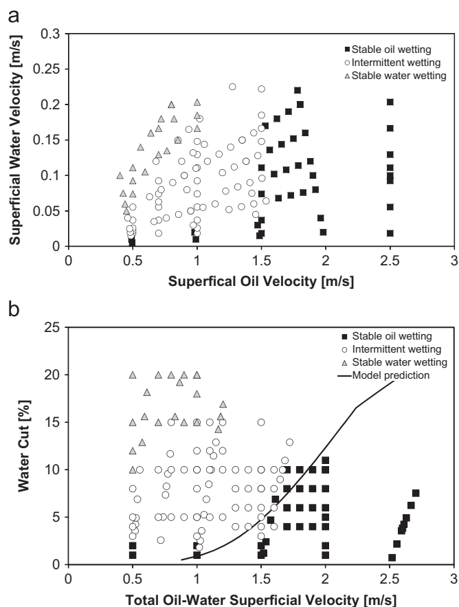
Fig. 10. Phase wetting map for LVT200 oil–water flow in large diameter (0.1 m) horizontal pipe. The data is displayed in two ways (a) using superficial velocities and (b) using water cut and the total oil–water superficial velocity. The model prediction is included in the latter.
